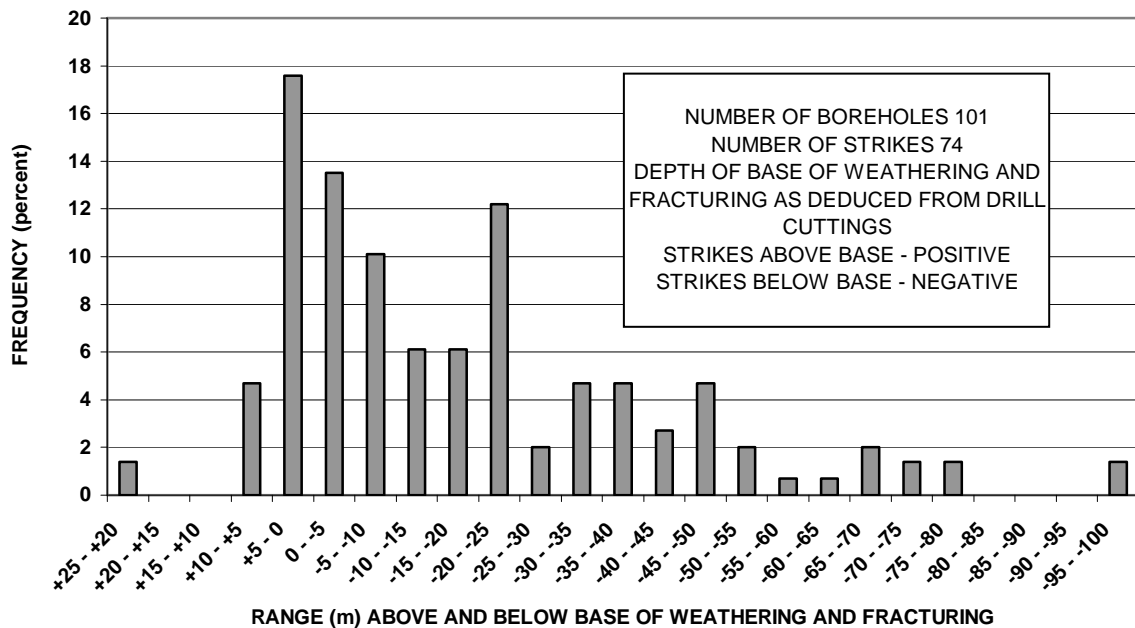
FIGURE 19 STRIKE FREQUENCY RELATIVE TO BASE OF WEATHERING AND FRACTURING BOLOBEDU
