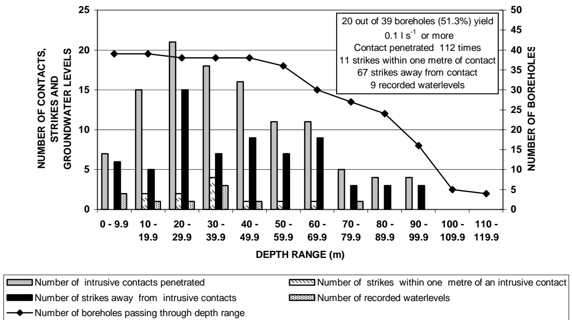
FIGURE 16 BOREHOLES PASSING SEVERAL TIMES THROUGH INTRUSIVE CONTACT
