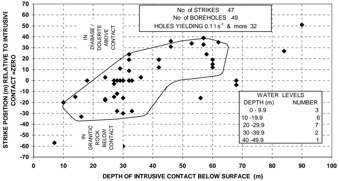
FIGURE 13 STRIKE POSITION RELATIVE TO INTRUSIVE CONTACT: BOREHOLES PASSING FROM DIABASE / DOLERITE INTO GRANITIC ROCK
